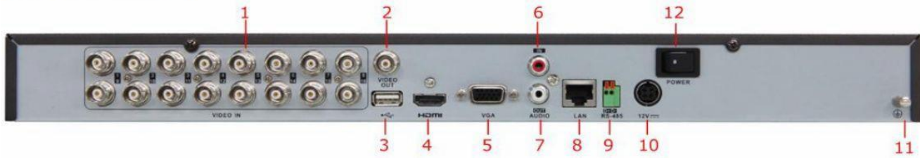
16 Channel Rear Panel
